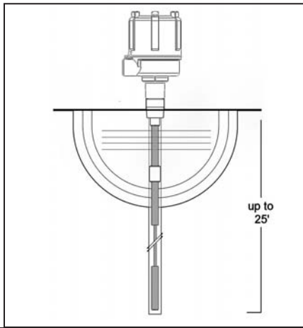
Shielded Teflon Sleeved 316 SS Hanging Flexible Cable Extension
